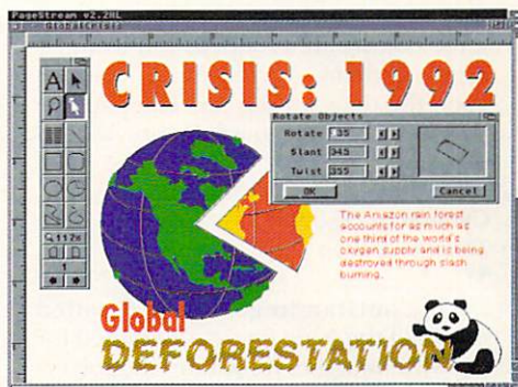
PageStream 2.2
